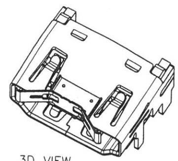
3D VIEW
